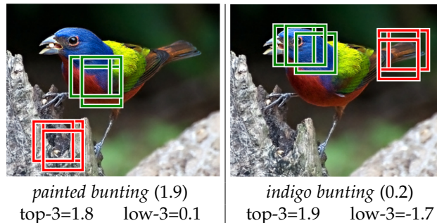
Fig. 3: Visual results of ResNet-WELDON with the final prediction score. We visualize the predicted regions for the ground truth model (left column) and a model of a similar incorrect class (right column). The top 3 positive (resp. top 3 negative) regions selected by the model are in green (resp. red).
