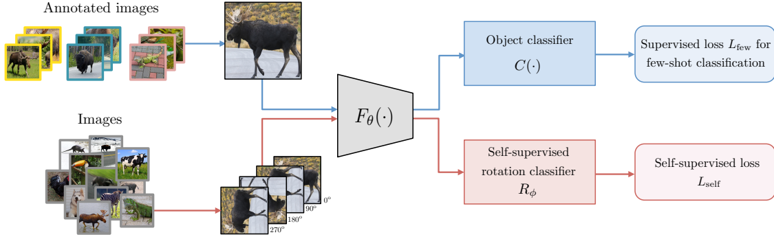
Figure 1: Combining self-supervised image rotation prediction and supervised base class recognition in the first learning stage of a few-shot system. We train the feature extractor F_\theta(\cdot) with both annotated (top branch) and non-annotated (bottom branch) data in a multi-task setting. We use the annotated data to train the object classifier C(\cdot) with the few-shot classification loss L_{\text{few}} . For the self-supervised task, we sample images from the annotated set (and optionally from a different set of non-annotated images). Here, we generate four rotations for each input image, process them with F_\theta(\cdot) and train the rotation classifier R_\phi with the self-supervised loss L_{\text{self}} . The pipeline for relative patch location self-supervision is analog to this one.
