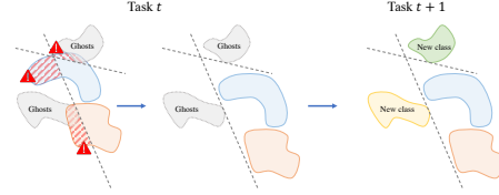
Figure 3: Latent-space regularization establishes margin-based one-unseen-class vs. all-seen-classes linear separations. Those separations are employed to directly condition the feature space, creating space for future unseen classes. In the following task, some unseen class will become seen, and may occupy the feature space with less interference.
