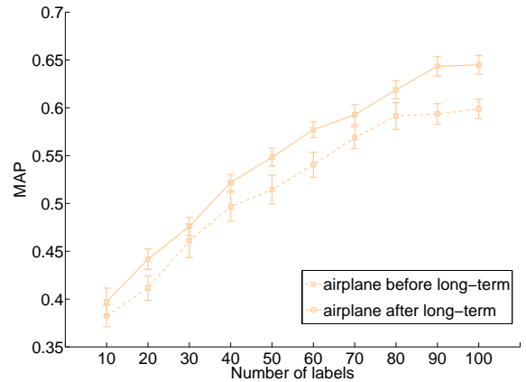
Fig. 8. MAP for the category airplane before and after learning. With the long-term optimization, the gain is about 5% and the speed-up is about 30 labels.
