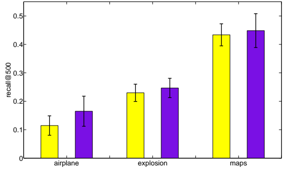
Fig. 7. Recall for each category for 500 images retrieved, compared to a classical CBIR system. The distributed system performs a little better on more difficult categories as airplane or explosion-fire .
