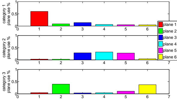
Fig. 6. Percentage of markers that were used for each category. Markers have been at most used for the category towards which destination they routed. For example, for the third category, the most used markers were the second and the sixth, which are leading to the host containing the third category as seen on Fig. 5
