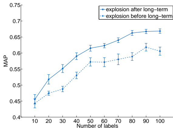
Fig. 10. MAP for the category explosion-fire before and after learning. With the long-term optimization, the gain is about 8% and the speed-up is about 60 labels.
