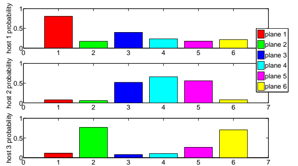
Fig. 5. Relative values of each marker on the three hosts. Each of the six planes has been specialized for one host. For example, the first plane has a higher probability to lead to the first host, while the second plane has a higher probability to lead to the third host.
