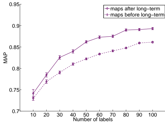
Fig. 9. MAP for the category maps before and after learning. With the long-term optimization, the gain is 5% and the speed-up is about 50 labels.
